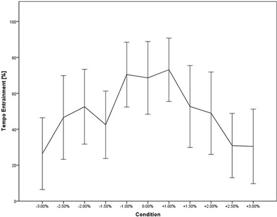
Fig. 4 Entrainment basin displaying mean tempo entrainment for the different conditions. Data presented is mean \pm 95 % CI
