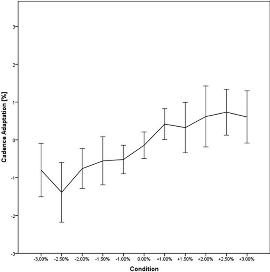
Fig. 1 Mean tempo and cadence adaptation for the different conditions. Data presented is mean \pm 95 % CI
